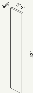
WF342 / WF642
