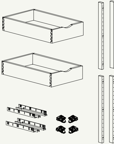
Roll Tray Kit Includes 2 x Roll Out Trays 2 x Sets of Soft-Close Slides 4 x Vertical Cleats And Screws
